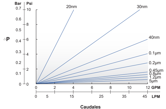
10" Polietersulfona Membrane Pleated Filter Cartridge
