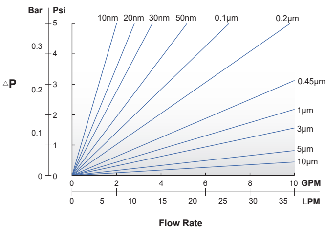
10" Hydrophilic PTFE Membrane Pleated Filter Cartridge
