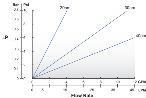
10" Polyethersulfone Membrane Pleated Filter Cartridge
