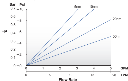
10" Nylon Membrane Pleated Filter Cartridge
