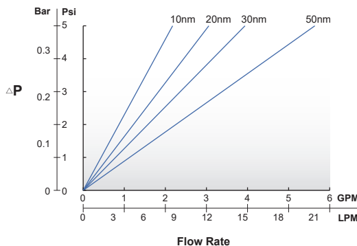
10" Hydrophilic PTFE Membrane Pleated Filter Cartridge
