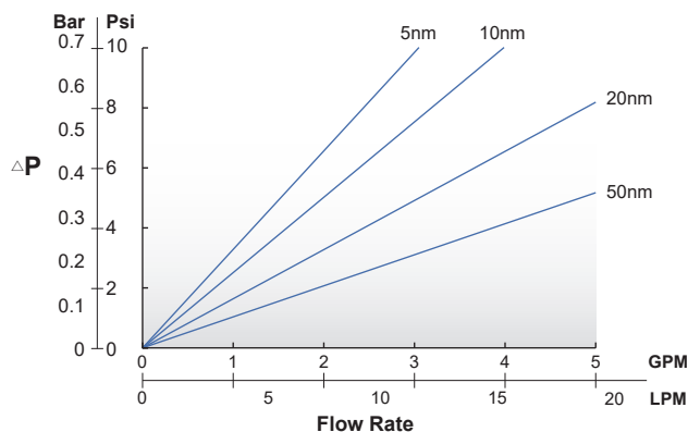
10" Nylon Membrane Pleated Filter Cartridge
