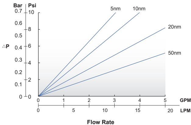
10" Nylon Membrane Pleated Filter Cartridge
